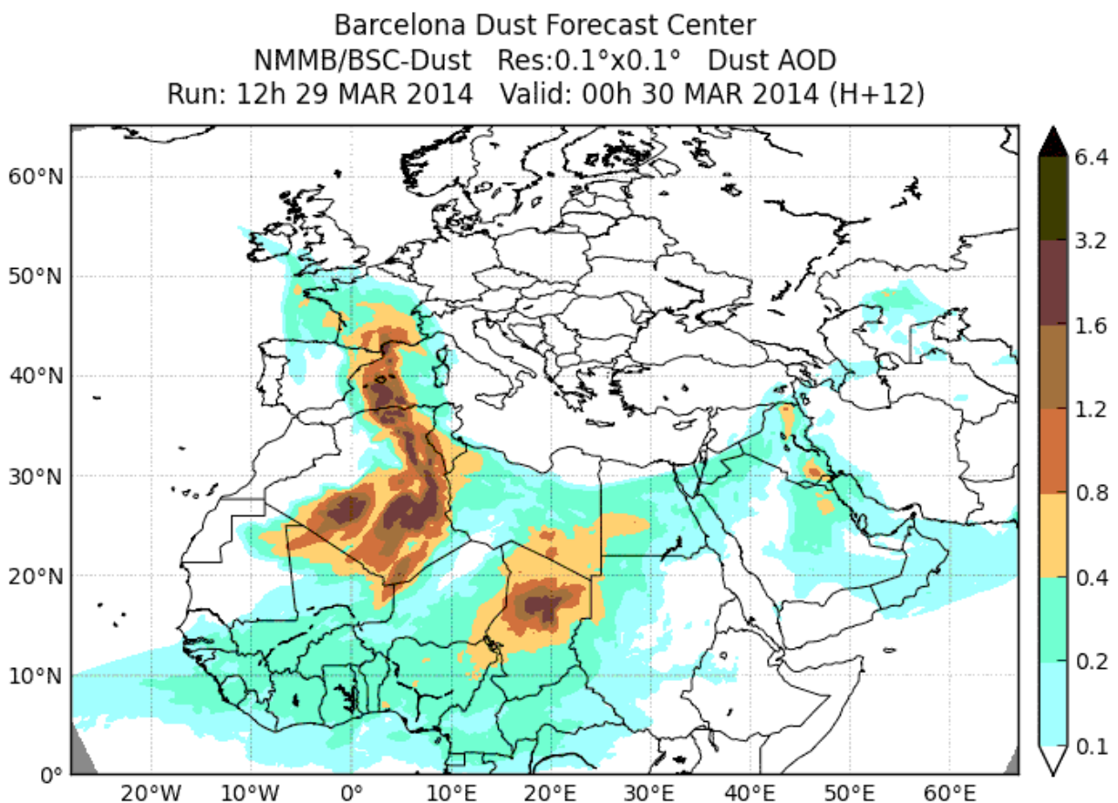
Figure 5.15: H+12 forecast of dust optical depth at 550 nm released by the Barcelona Dust forecast Centre on 29 March 2014 at 12 UTC. Source: Barcelona Dust Forecast Center.
