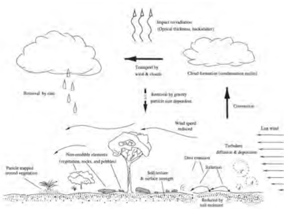
Figure 2.2: A simplified depiction of sand and dust storm processes, controlling factors and impacts. Source: Lu and Shao 2001.
