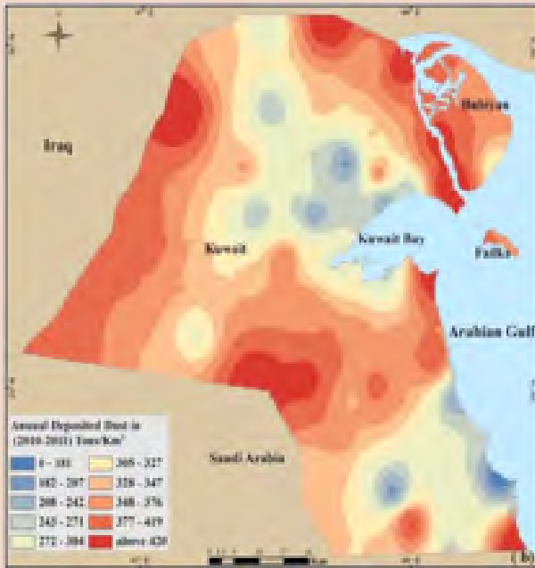
Annual dust fallout in Kuwait 2010-2011
