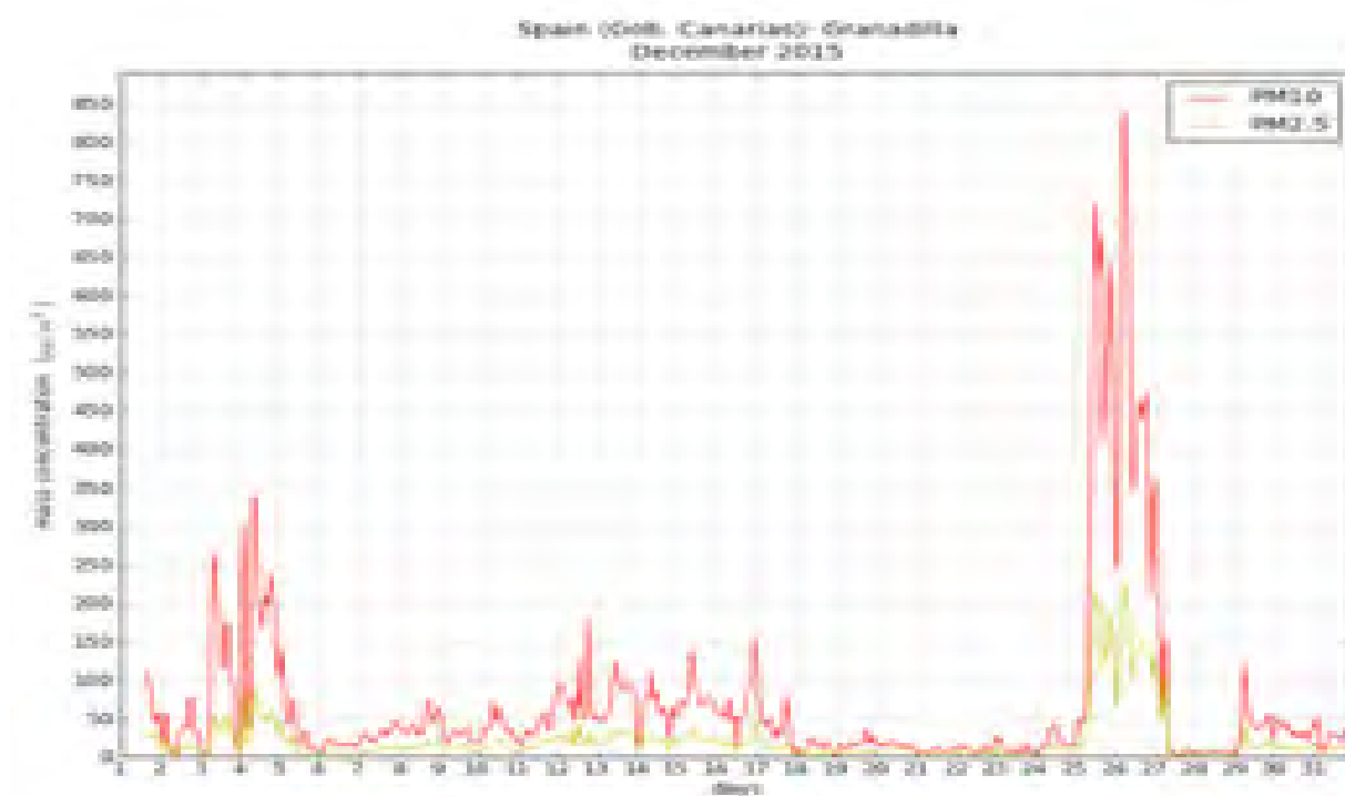
Figure 5.2: The record of particulate matter of 10 µm or less in diameter (PM 10 ) and 2.5 µm in diameter (PM 2.5 ) from Granadilla (Canary Islands, Spain), which clearly shows a major dust event on 25-26 December 2015 and a less significant one on 4-5 December. Source: SDS-WAS.
