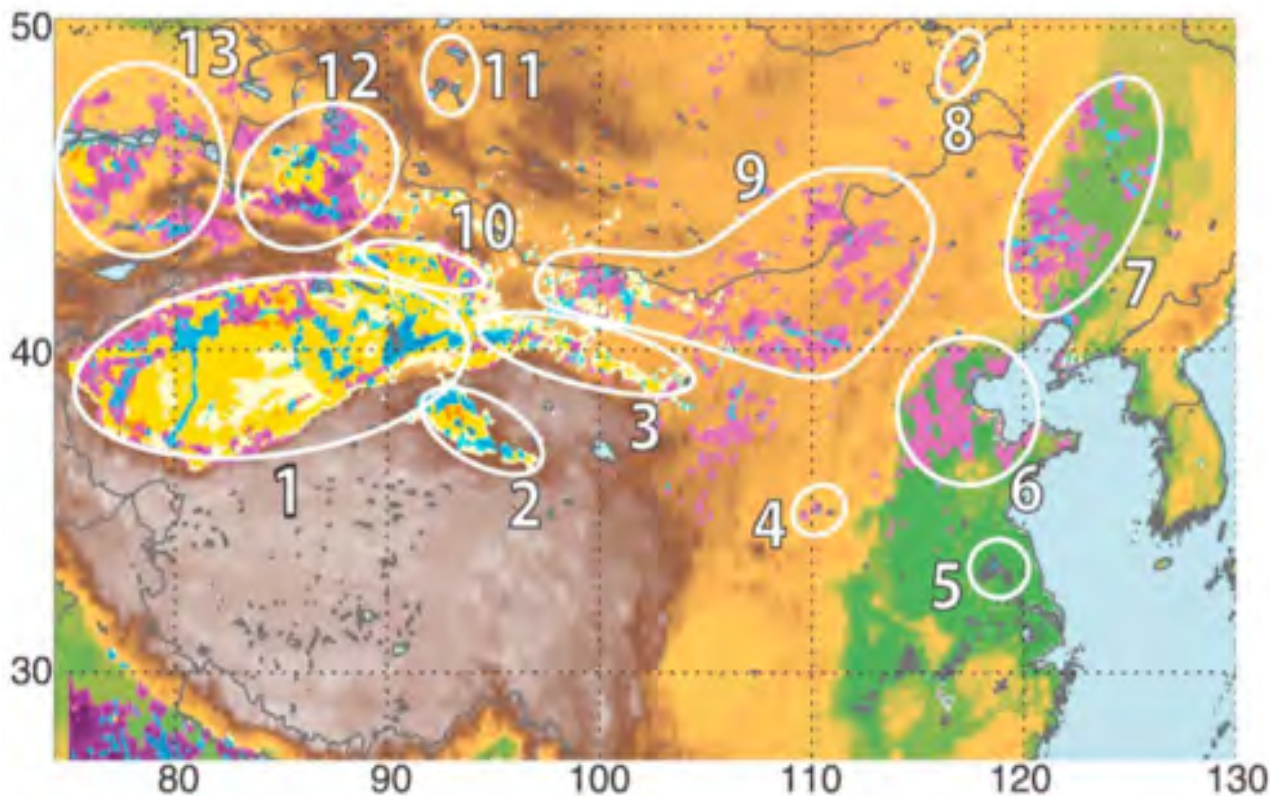
Figure 3.13: Distribution of the percentage number of days per season (March, April, and May) with Dust Optical Depth > 0.2 over East Asia. The colour shadings are the same as in Figure 35. The white circled source areas are numbered as follows: 1, Tarim Pendi; 2, Qaidam Pendi; 3, Hexi corridor in Gansu Province; 4, Tongguan county; 5, Hongze and Gaoyou Lakes of eastern China; 6, North China Plains; 7, Horqin sandy land; 8, Hulun Buir plain; 9, Inner Mongolia deserts; 10, Turpan Pendi; 11, Great Lakes depression in Mongolia; 12, Junggar Pendi; and 13, Balkhash-Alakol depression. Source: Ginoux et al. (2012).
