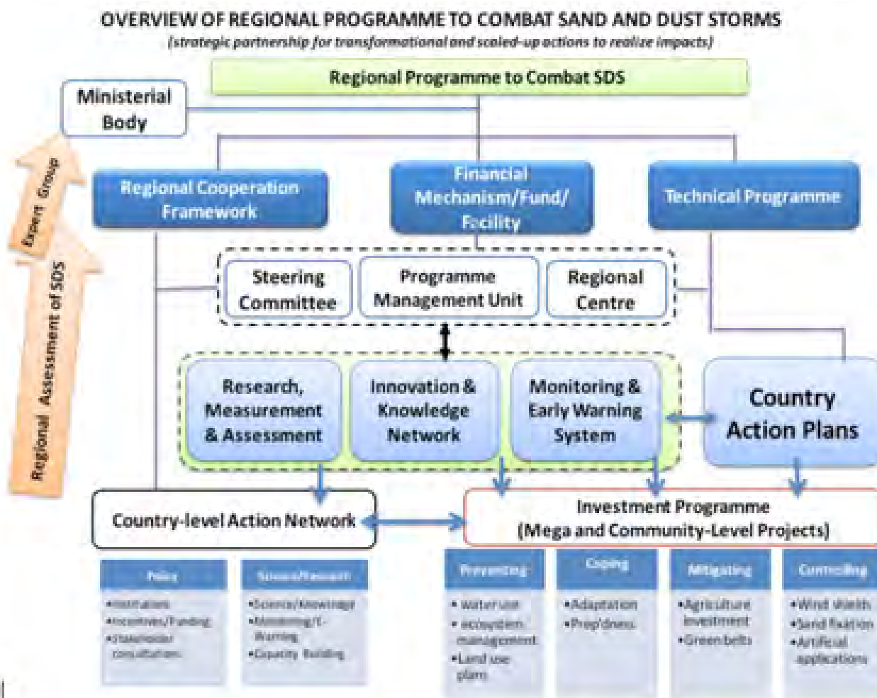
Figure 71: Overview of West Asia regional programme to combat sand and dust storms. Source: UNEP (2014).
