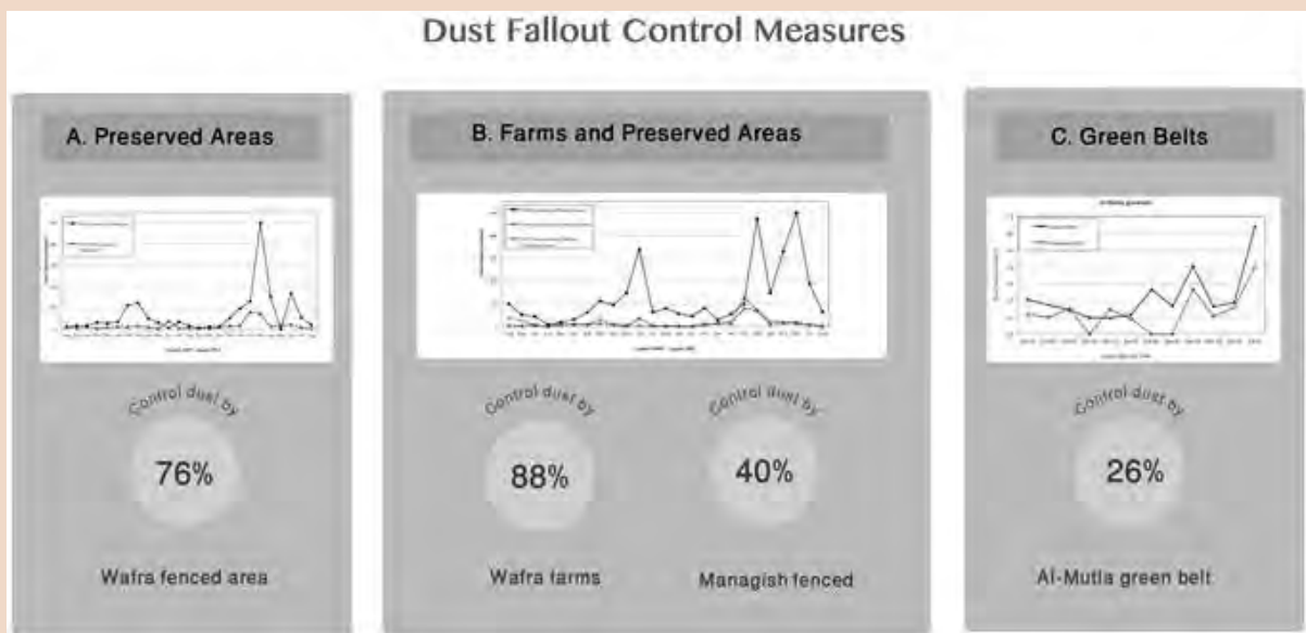
Line plots showing dust deposition rates and reduction percentages (circles) in downwind areas compared to upwind areas for fenced areas (a) farms and fenced areas (b) and green belts (c).
