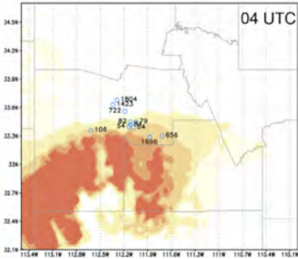
Figure 5.17: NMME DREAM 16 hour hindcast of a 5 July 2011 haboob through Phoenix, Arizona, USA. PM 10 near surface concentrations ( \mu\text{g}_\text{m}^{-3} ); spatial resolution ~ 3.5km. Source: Vukovic et al. 2014; Sprigg et al. 2014.
