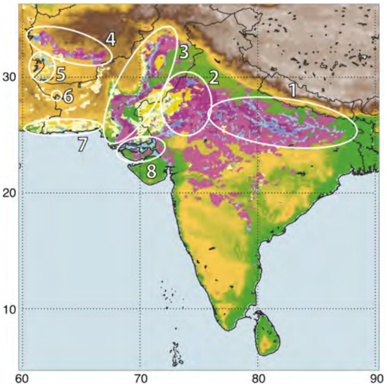
Figure 3.12: Distribution of the percentage number of days per season (March, April, and May) with Dust Optical Depth > 0.2 over South Asia. The colour shadings are the same as in Figure 35. The white circled sources are numbered as follows: 1, Ganges basin in India; 2, desert of Rajasthan in India; 3, Indus basin of Pakistan; 4, southern drainage basin of the Hindu Kush in Afghanistan; 5, ephemeral lakes around the city of Zabol; 6, Hamun-i-Mashkel of Pakistan; 7, Makran coast of Pakistan; and 8, Rann of Kutch in India. Source: Ginoux et al. (2012).
