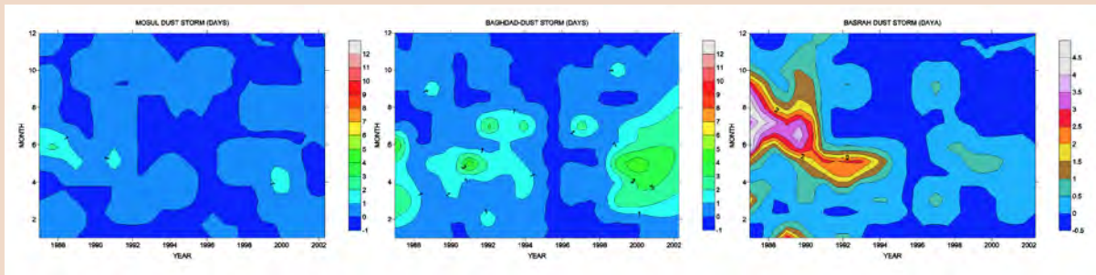
Contour map of dust storms for Mosul, Baghdad and Basra and for the period 1987-2002. Source: Abdulkareem et al. 2013.
