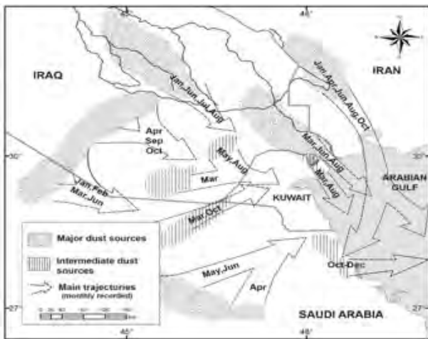
Figure 3.7: Major and intermediate source areas and trajectories for dust storms in the north-western areas of Persian Gulf based on dust storm days in Kuwait and satellite images from 2000 to 2010. Source: Al-Dousari & Al-Awadhi (2012).
