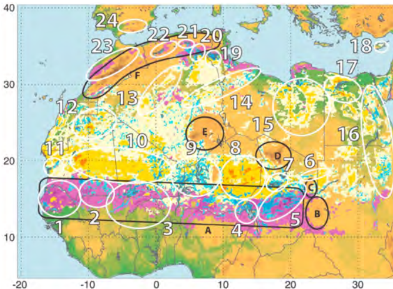
Figure 3.5: Distribution of the percentage number of days per year with Dust Optical Depth > 0.2 over West and North Africa and Southern Europe. The frequencies associated with hydrologic sources are shaded in blue, with natural land use in yellow to red, and anthropogenic land use (more than 30%) in magenta. The frequency levels are 10%, 20%, 40%, 60%, and 100%. Topography shading varies from dark green (300 m) to brown (1000–4000 m), then to grey for high elevation up to 8000 m. The white circled source areas are numbered as follows: 1, Senegal River Basin; 2, Aoukar depression; 3, upper Niger River Basin; 4, Lake Chad; 5, river drainage basin of the Ennedi and Ouaddai highlands; 6, Mourdi depression; 7, Bodélé depression; 8, Grand Erg of Bilma; 9, river drainage basin of the Aïr; 10, Erg El Djouf; 11, Sebket te-n-Dgâmcha; 12, Tiris Zemmour region; 13, Grand Erg Occidental; 14, Grand Erg Oriental; 15, Libyan Desert; 16, Nile River Basin; 17, Qattarah depression; 18, Mesaoria plain in Cyprus; 19, Chott el Jerid; 20, Chott Melrhir; 21, Chott el Hodma; 22, Chott ech Chergui; 23, Morocco coastal plains; and 24, Andalusia in Spain. Some geographic features are contoured in black and are labeled as follows: A, the Sahel; B, the Ouaddai Highlands; C, Ennedi; D, Tibesti; E, Ahaggar; and F, Atlas Mountains. Source: Ginoux et al. (2012).
