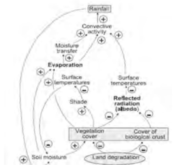
Figure 2.7: Land degradation and climate regulating process (MA 2005a). Positive signs indicate enhancing effects, while negative signs indicate reducing effects.
