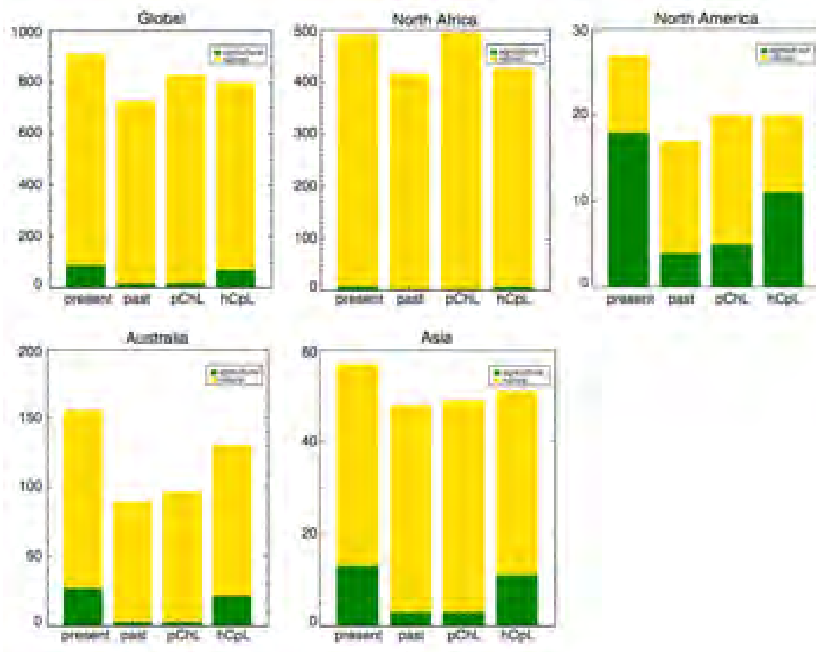
Figure 2.9: Integrated 10 year mean (2000–2010) annual dust emission flux in Tg/year for different regions as simulated in present, past, present climate historical land use (pChL), and historical climate present land use (hCpL). Dark green denotes emissions from agricultural source regions and yellow emissions from natural source regions. Note the use of different axis ranges. Source: Stanelle et al. (2014).
