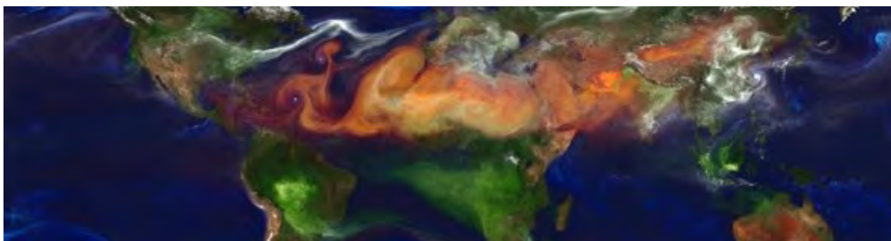
Figure 3.1: Atmospheric Aerosol Eddies NASA Animated Map: 10km GEOS-5 Aerosol Optical Depth (AOD): Red/yellow colours – Dust Aerosols. Source: NASA (2014).
